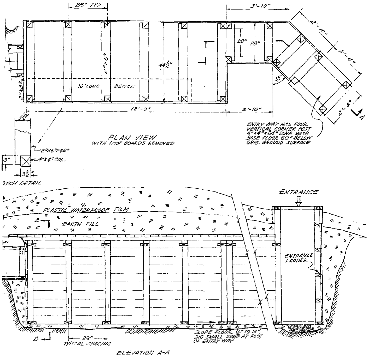
A-5.1. Shored Trench Stoop-In Shelter, Plan and Elevation.
